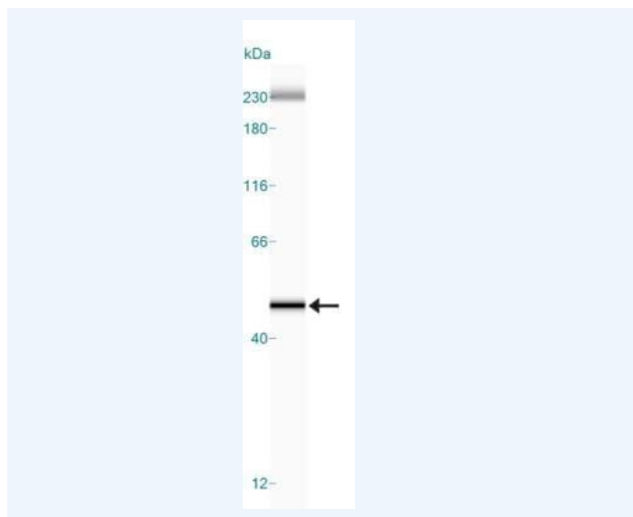
Figure1 Simple Western: Actin Antibody (mAbGEa) [NB100-74340] - Image shows a specific band for Actin in 0.1 mg/mL of HeLa lysate. This experiment was performed under reducing conditions using the 12-230 kDa separation system.
