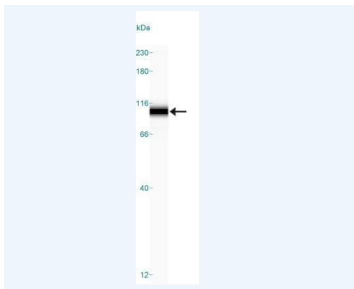
Figure1 Simple Western: ATF6 Antibody [NBP1-75478] - Simple Western lane view shows a specific band for ATF6 in 1.0 mg/ml of HeLa lysate. This experiment was performed under reducing conditions using the 12-230kDa separation system.
